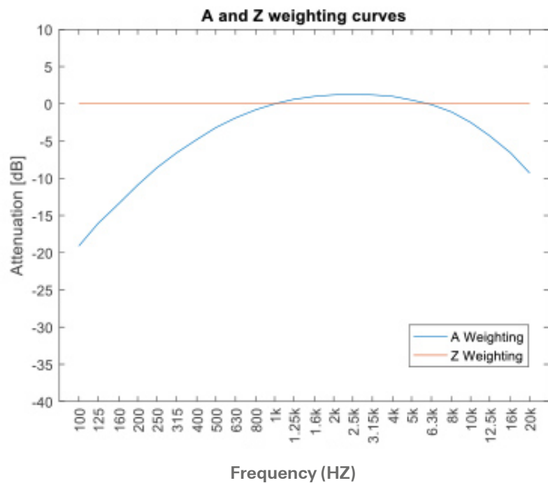
Figure 6: One-third octave band frequency domain depiction of A and Z weighting.
