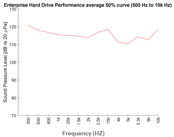
Figure 4: The SPL at one third octave frequency bands where the performance of the HDD was reduced by 50 % from the baseline values. The plot in the red shows the average of the 50 % points for 12 different HDDs.
