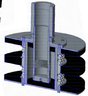
Figure 9: Acoustic Nozzle Section View
