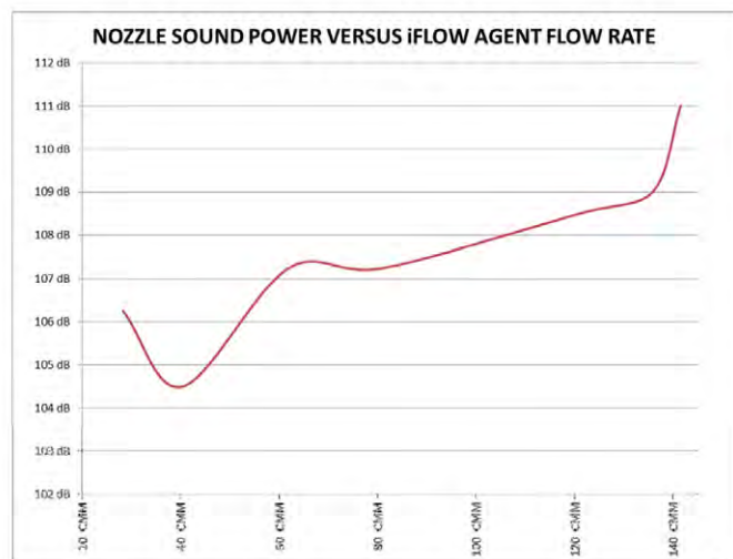
Figure 11: The peak sound power vs flow rate for Tyco's acoustic nozzle (m 3 /min flow rates)
