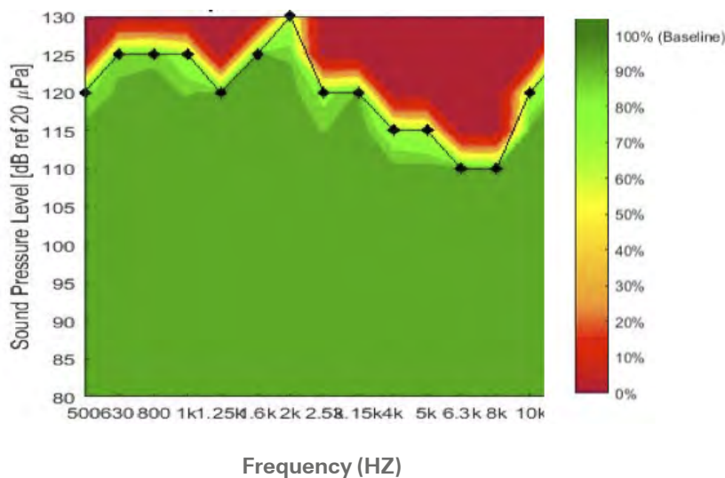
Figure 3: The minimum read and write speeds as percentage of their respective baseline values shown in OTO frequency bands. The performance of the HDD drops dramatically after reaching the 50% curve shown by the black curve with black diamond data points.
