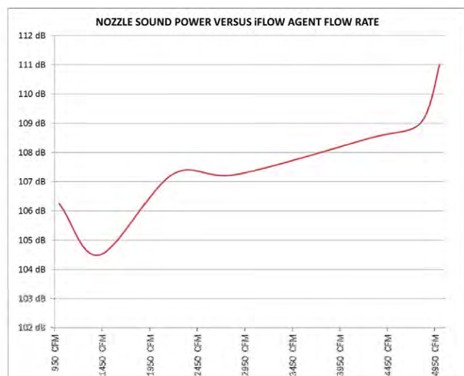
Figure 12: The peak sound power vs flow rate for Tyco's acoustic nozzle (CFM flow rates)
