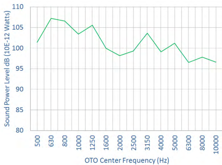
Figure 10: The sound power at one third octave frequency bands for Tyco's Acoustic Nozzle, tested with the iFLOW system with a nozzle agent flow rate of 61.9 m 3 /min (2188 CFM).
